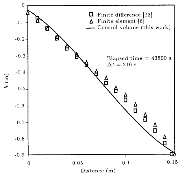
Figure 8. Water pressure head (m) along the length of the soil at a distance of 0.005 m below the top ( \Delta x = 0.01 m, \Delta y = 0.005 m).
